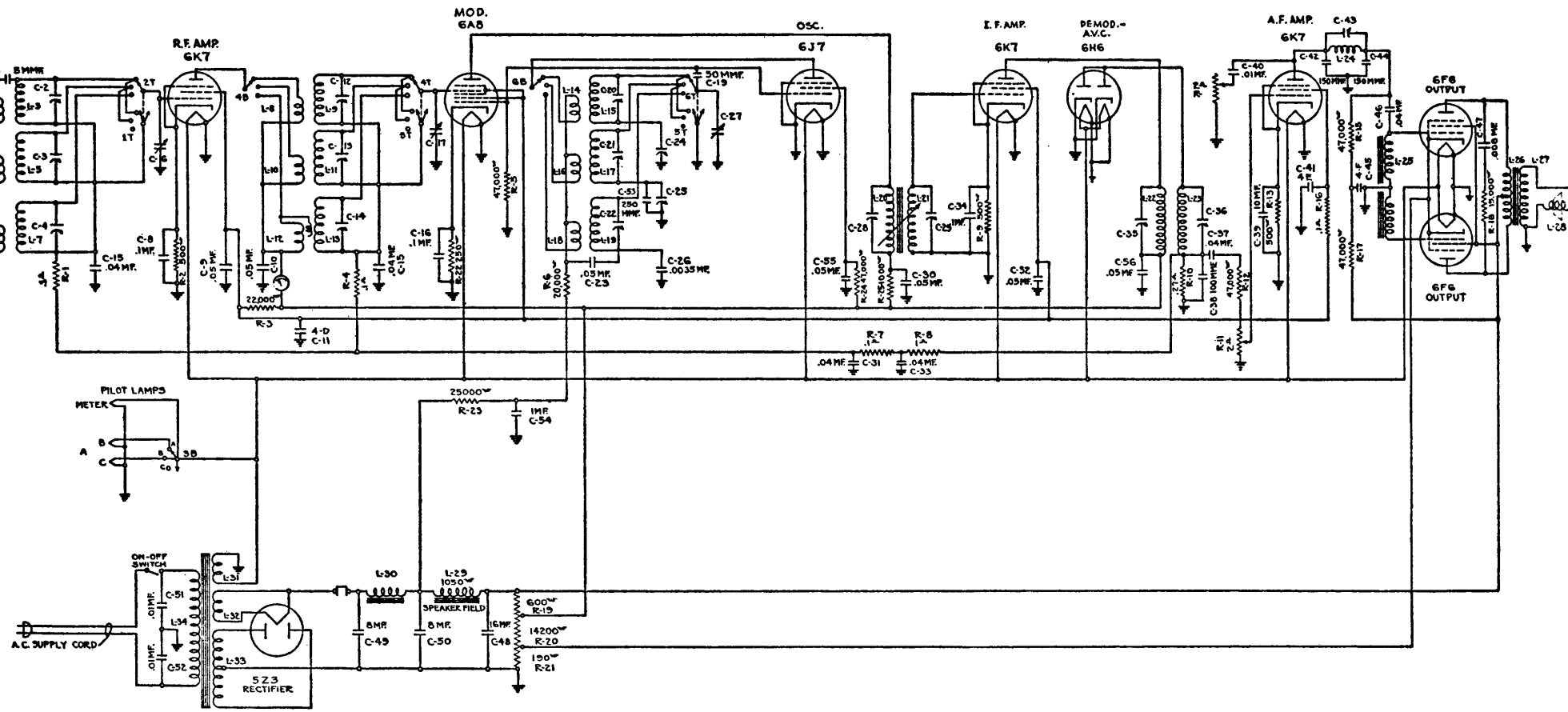
Fig. 2. Schematic Circuit of Receiver.
